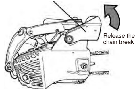
Front hand guard
